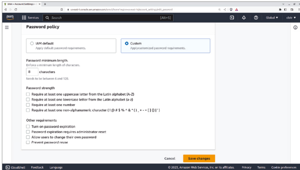
FIGURE 5.1 The IAM Account Settings page where you can set an account-wide password policy
