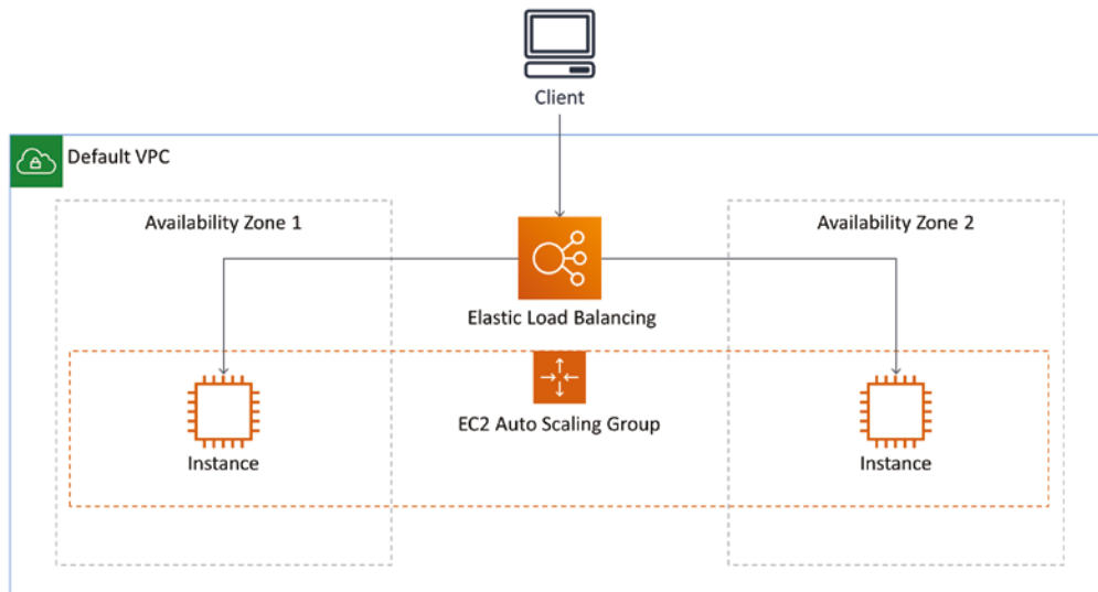
FIGURE 12.1 A highly available web application using Auto Scaling and elastic load balancing
